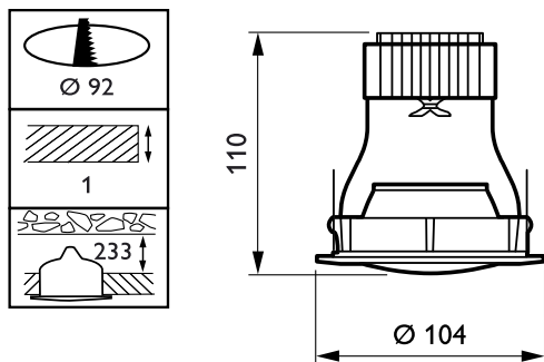
Smart halogen downlight QBS040
