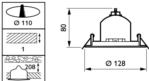
Smart halogen downlight QBS020
