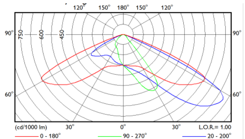
BRP042 LED19 CW MR S1 PSU GR.PHL
